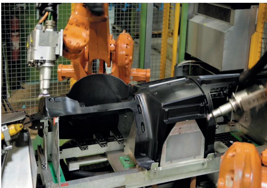
Fig. 5. Activating the surface with plasma technology increases the surface energy and improves the adhesion of adhesives and paints, even with plastic parts made from recycled material. © Plasmatreteat
